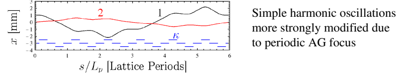
Simple harmonic oscillations modified with additional harmonics due to periodic focus
