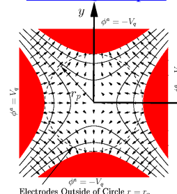
Electrodes Outside of Circle r = r_p Electrodes: x^2 - y^2 = \pm r_p^2
