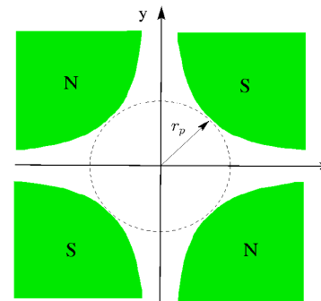
Hyperbolic Iron Pole Sections (infinite)
