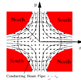
Conducting Beam Pipe: r = r_p Poles: xy = \pm r_p^2
