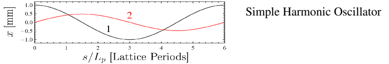
Simple harmonic oscillations modified with additional harmonics due to periodic focus
